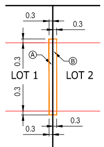
PARTY WALL EASEMENT TYPICAL DETAIL NOT TO SCALE
