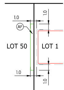
MAINTENANCE EASEMENT TYPICAL DETAIL NOT TO SCALE
